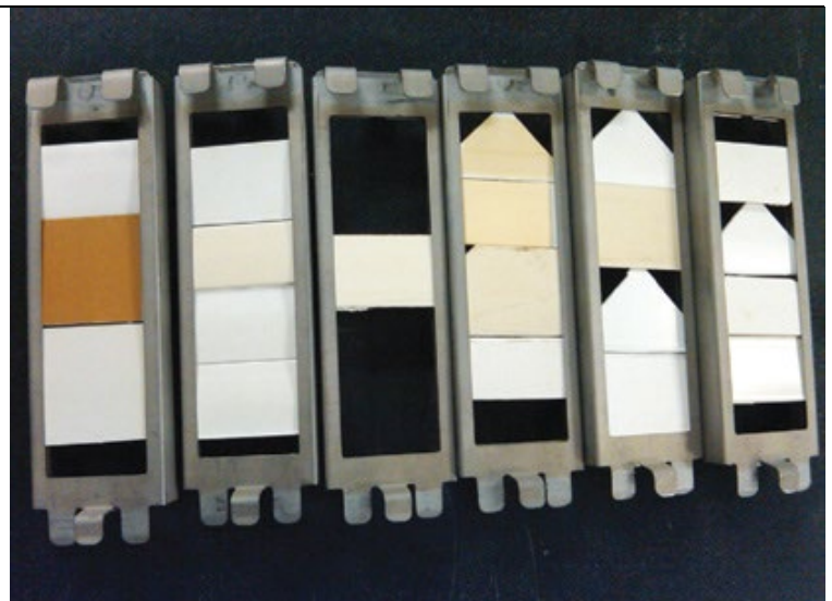
Accelerated Weather Test
